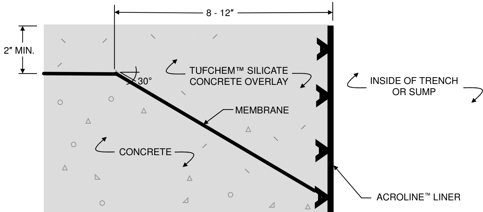
ELEVATION VIEW
